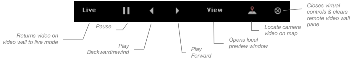
Figure 113 Video Wall Controls
