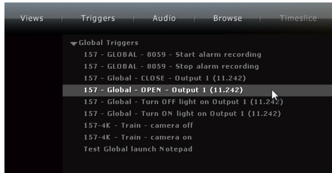
Figure 99 Manually Execute a Global Trigger
