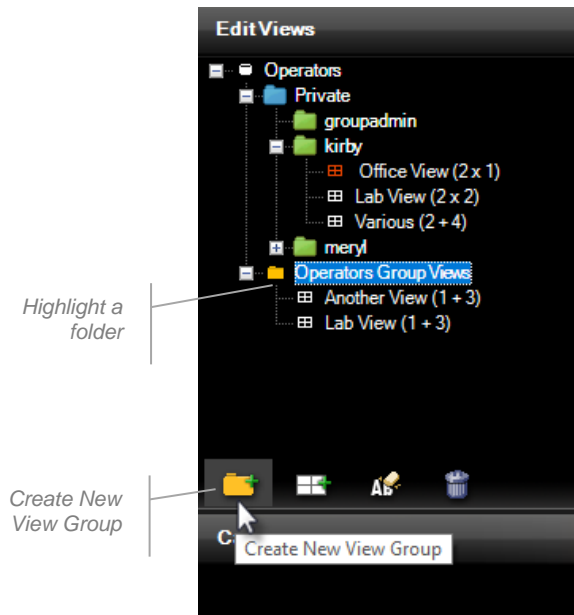
Figure 18 Edit Views Using Ocularis Client
